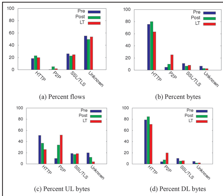
Figure 7. Tstat analysis of service types.
