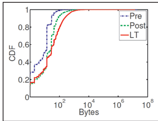
Figure 5. Bytes in flight.
