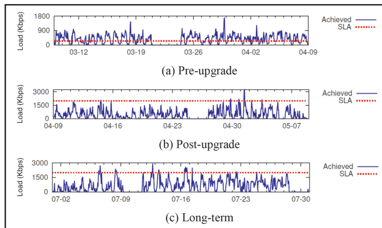
Figure 2. Traffic load over time
