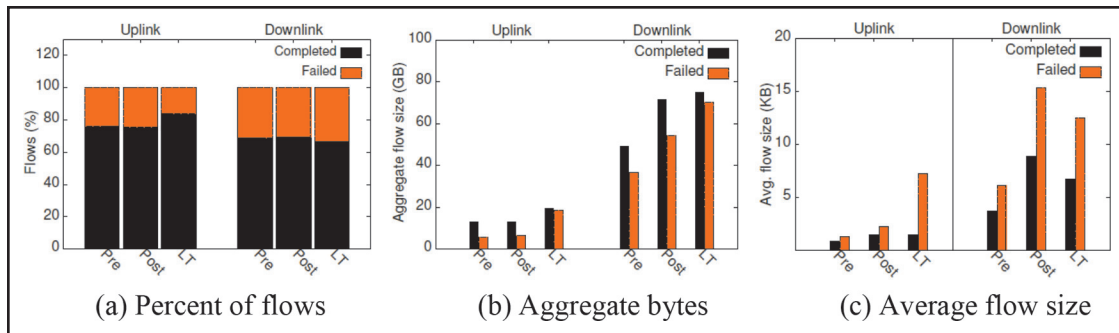
Figure 6. TCP flow success and failure in uplink and downlink directions.
