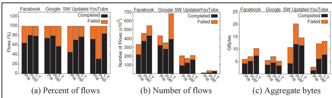
Figure 9. TCP flow success and failure for URIs of interest.
